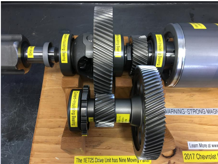
Chevy Bolt EV single speed gear box
